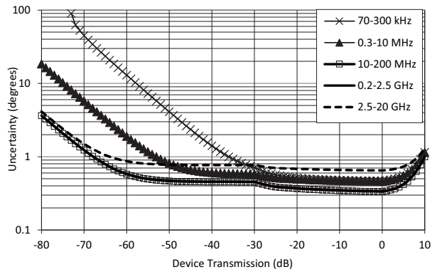
Transmission Phase Uncertainty; MS4642B (Opt. 61/62); SOLT- SL Calibration using 3652A -1 K kit
