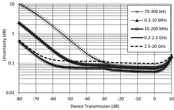
Transmission Magnitude Uncertainty; MS4642B (Opt. 61/62); SOLTSL Calibration using 3652A -1 K kit
