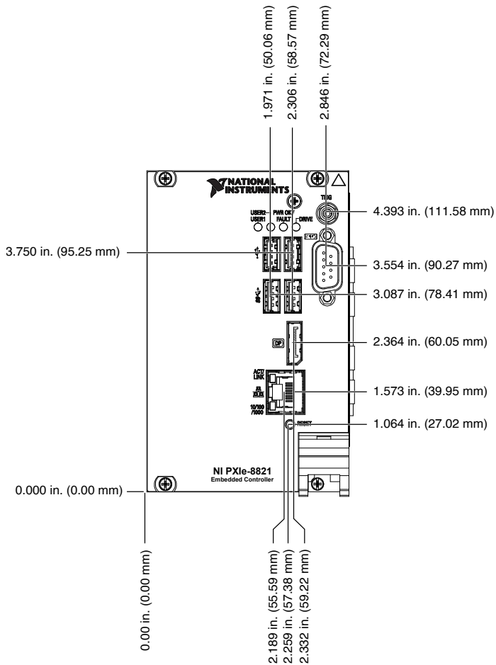
Figure 1. PXIe-8821 Front Panel Layout and Dimensions
