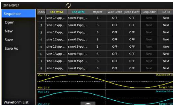
Figure 2: Advanced mode lets you build complex waveform sequences with flexible step controls
