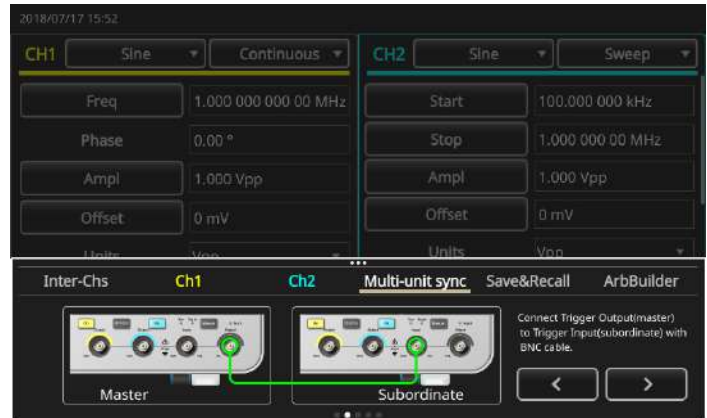
Figure 8: An on-screen wizard guides you through the process of multiple-unit synchronization
