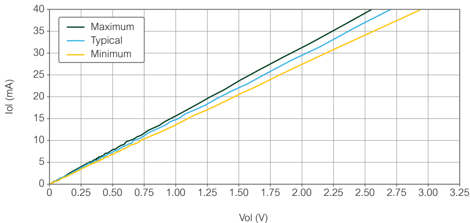
Figure 7. I_{OL} versus V_{OL} , 5.0 V Logic Family
