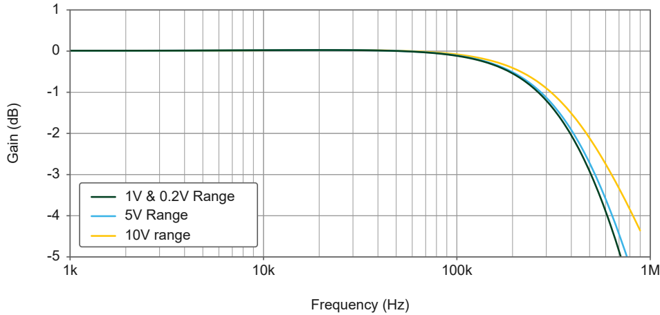
Figure 3. USB-6421 Small Signal Bandwidth versus Frequency
