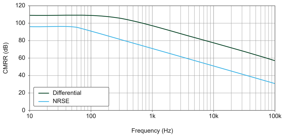
Figure 4. USB-6421 CMRR versus Frequency
