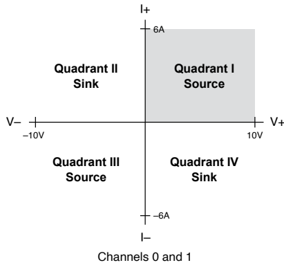
Figure 1. PXle-4113 Quadrant Diagram
