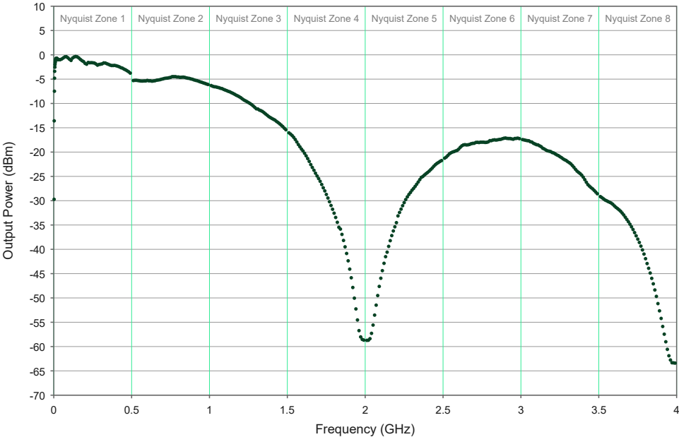
Figure 1. TX Maximum Output Power: 0 dBFS CW, 2.94912 GSps Converter Rate, 0 Hz Waveform
