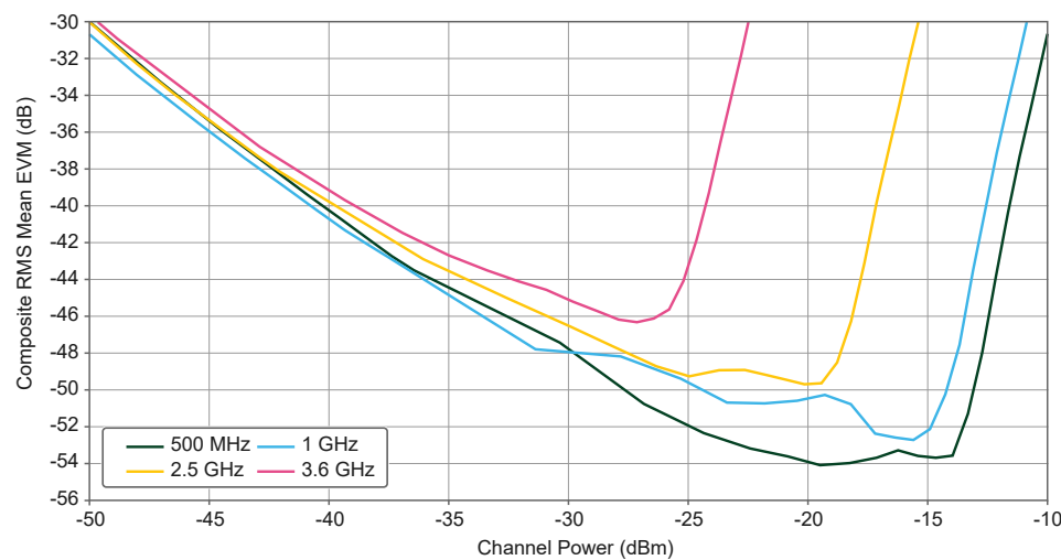
Figure 1. TX EVM Bathtub Curves: 5G NR, UL, FDD, SISO, 100 MHz BW, 30 kHz SCS, 256 QAM
