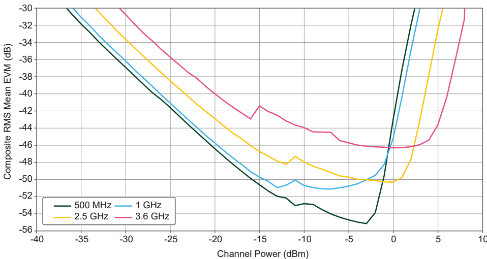
Figure 1. RX EVM Bathtub Curves: 5G NR, UL, FDD, SISO, 100 MHz BW, 30 kHz SCS, 256 QAM
