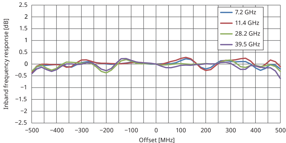
Inband frequency response without MS2850A-068 (meas.)
