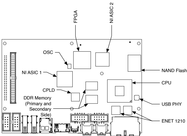
Figure 5. sbRIO-9629 Component Locations
