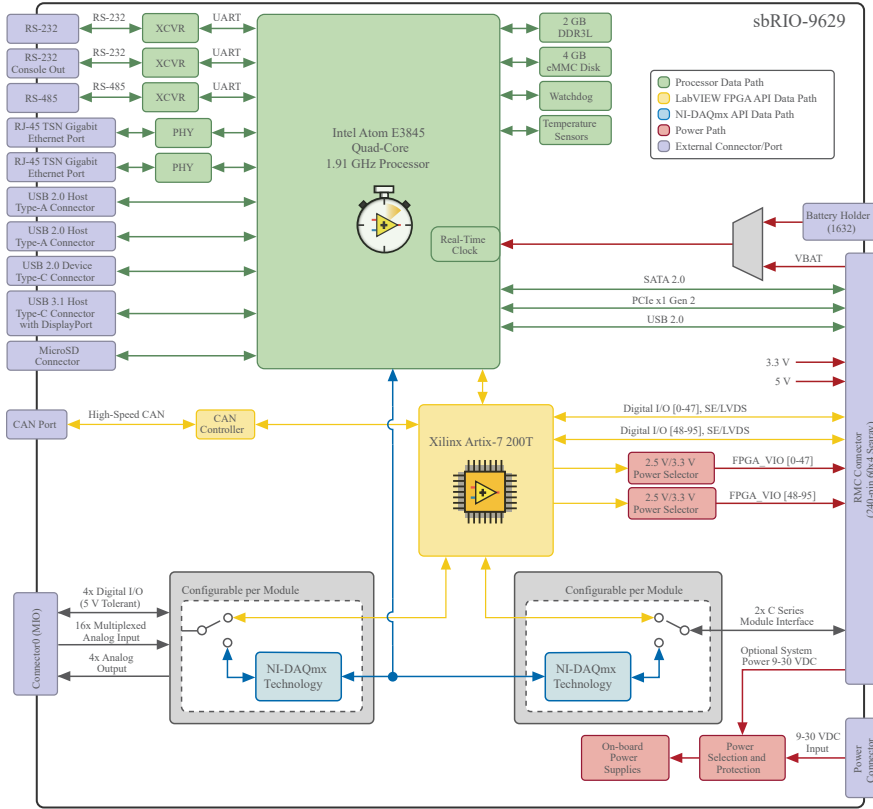
Figure 1. sbRIO-9629 Block Diagram
