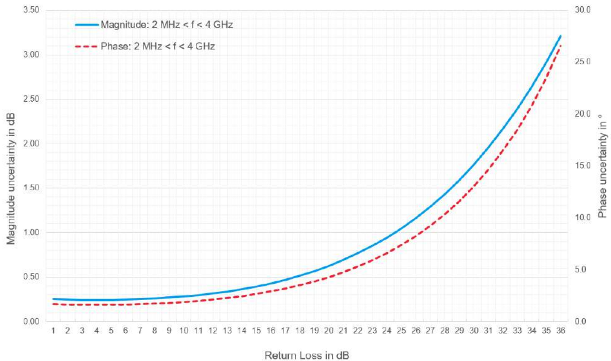
Uncertainty of reflection measurements with R&S®ZN-Z103 Temp: +18 °C to +25 °C, RBW: 10 Hz, Power: -10dBm
