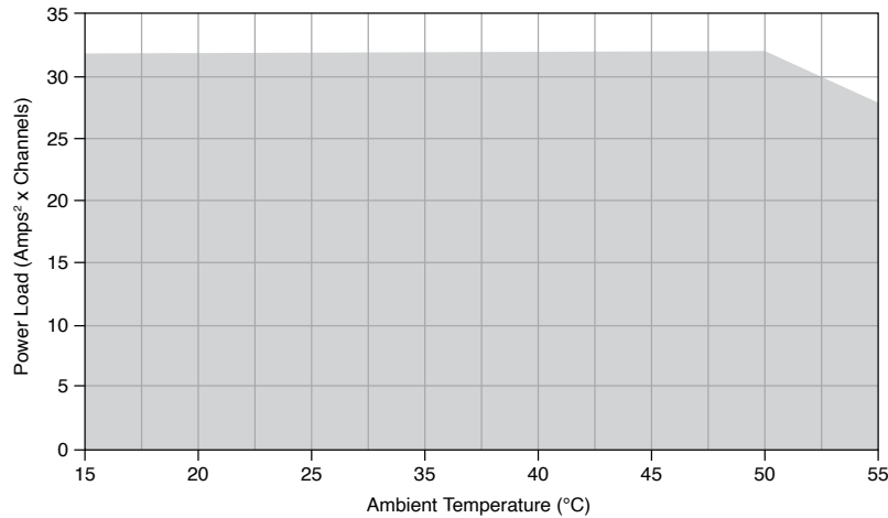
Figure 1. PXIe-2738 Load Derating, 2-Wire
