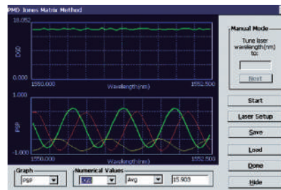
DGD and PSP measurement (Jones Matrix Eigenanalysis) of two 15.75 mm YVO 4 crystals with 45° alignment. Specified DGD=15.90ps, SOPMD=126.46ps 2 , Measured DGD=15.903ps
