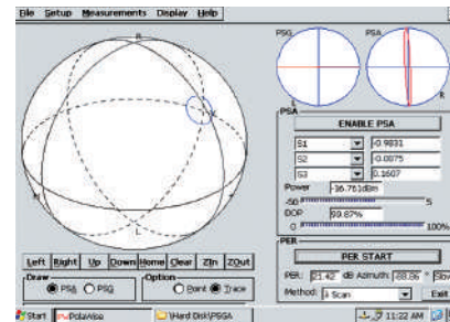
PER measurement example. The PM fiber under test has a PER of 21.42 dB, and the key of the PM output connector is aligned 1.1° from the slow axis of the fiber.
