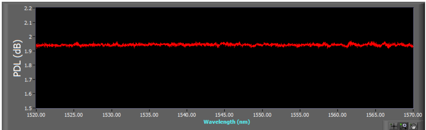
Figure 4. PDL vs. wavelength for a 1.96dB PDL artifact. The data indicates that the PDL of this device is relatively flat over the tested wavelength range.
