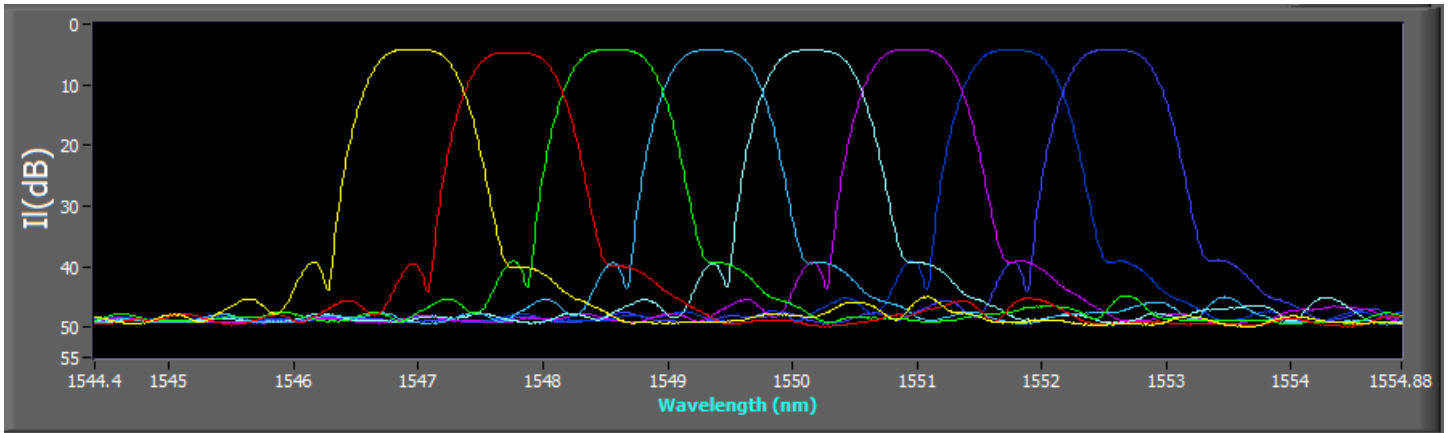
Figure 1. IL vs. wavelength for 8 channels of an arrayed waveguide grating (AWG). Pass bands for each channel are clearly visible.
