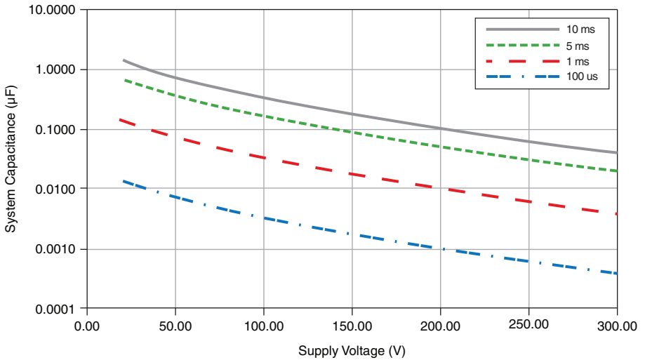
Figure 6. NI-9437 Capacitance Tolerance
