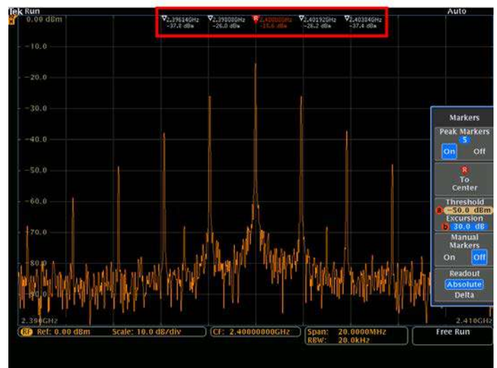
Automated peak markers identify critical information at a glance. As shown here, the five highest amplitude peaks that meet the threshold and excursion criteria are automatically marked along with the peak's frequency and amplitude.
