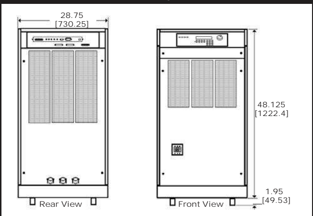
MX22.5/30/MX45 Dimensions - single chassis
