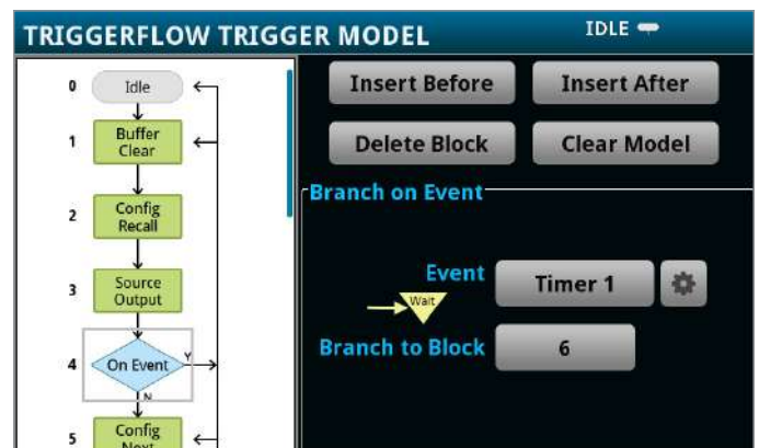
TriggerFlow building blocks allow creating triggering models that range from very simple to highly complex.
